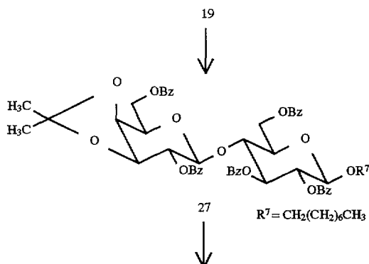
Reaction Scheme 3
