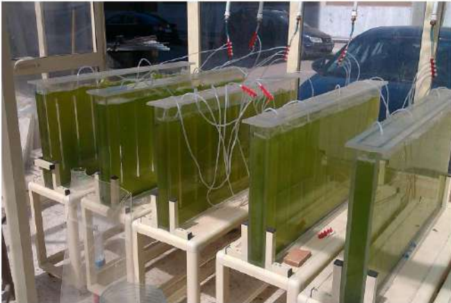
Algae Cultivated In Flat Panel Photo-Bioreactor, Med-Algae Project (Faculty of Science, Alexandria University)
